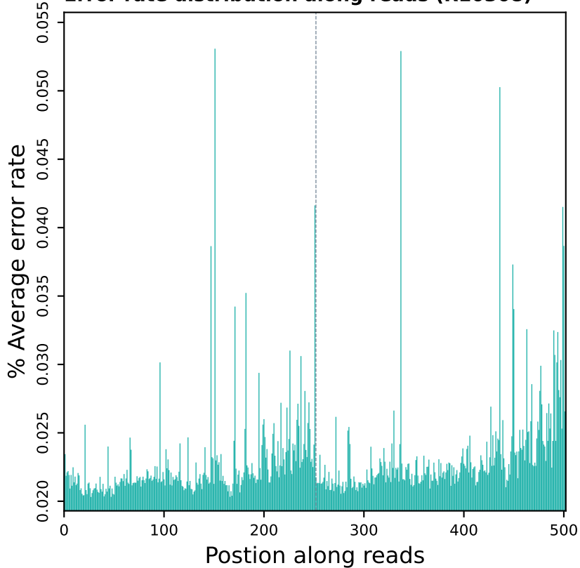
Error rate distribution along reads (R10308)
